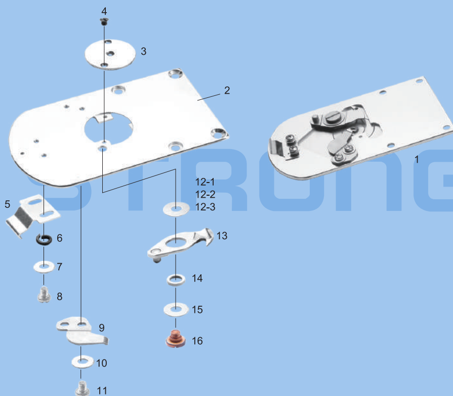
BAS-311G 剪线组件 ASSEMBLY FOR BAS-311G
